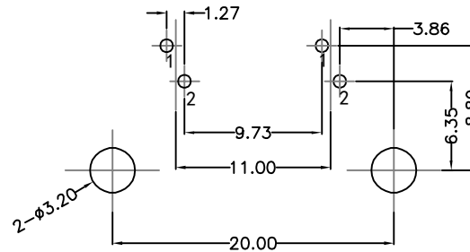
RECOMMENDED PCB LAYOUT VIEWED FROM COMPONENT SIDE
